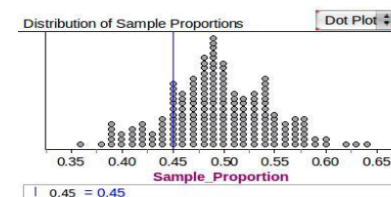
Population proportion 0.5; sample size
