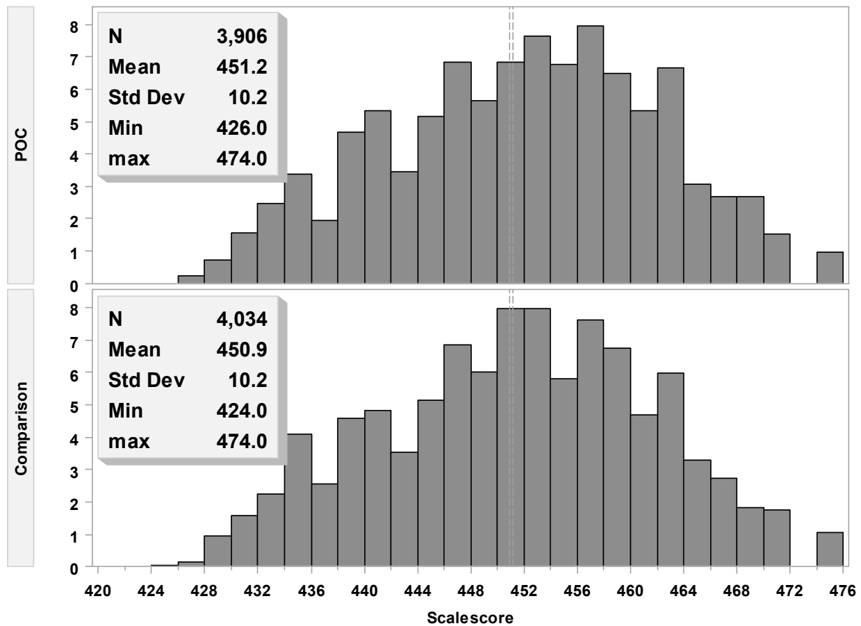
Figure 15. Scale score comparison between the POC and comparison samples—grade 5 math
