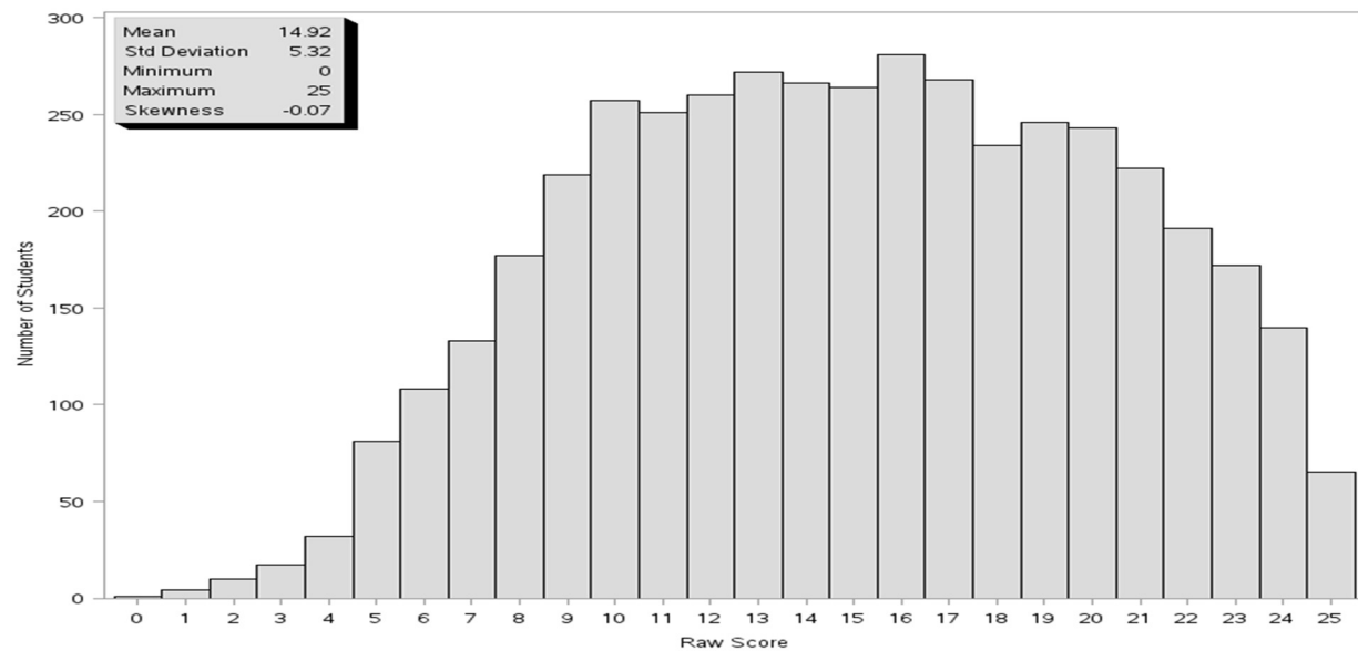
Figure 7. Raw score frequency distribution of grade 5 math interim 1
