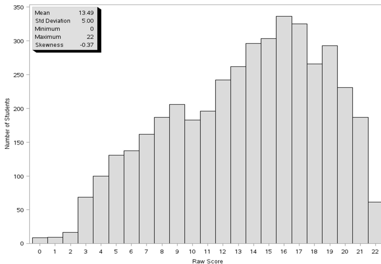
Figure 8. Raw score frequency distribution—grade 6 ELA/reading interim 2
