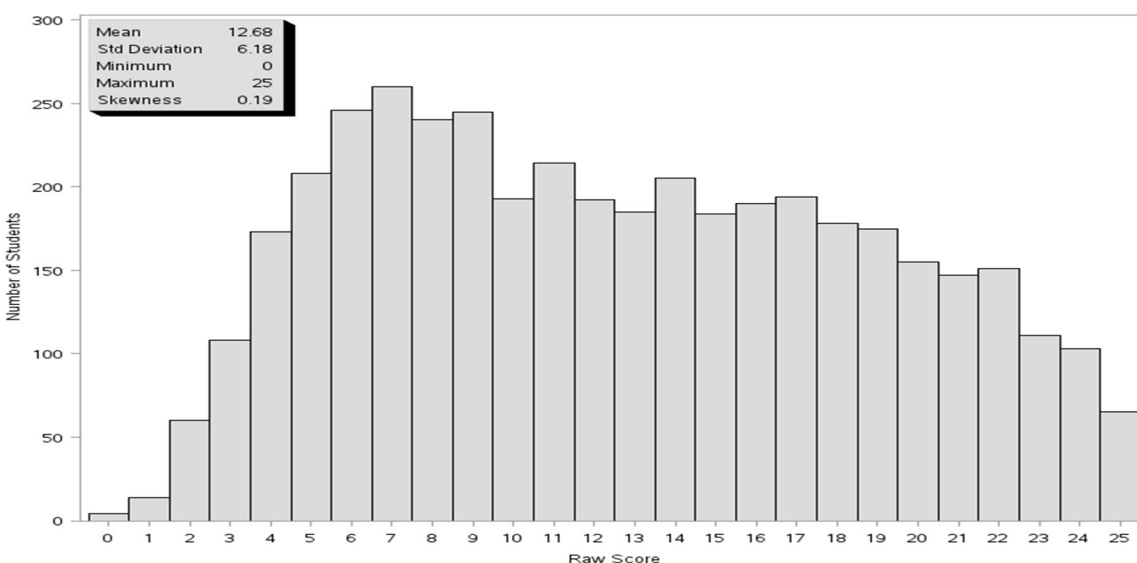
Figure 13. Interim 3 raw score frequency distribution—grade 5 math
