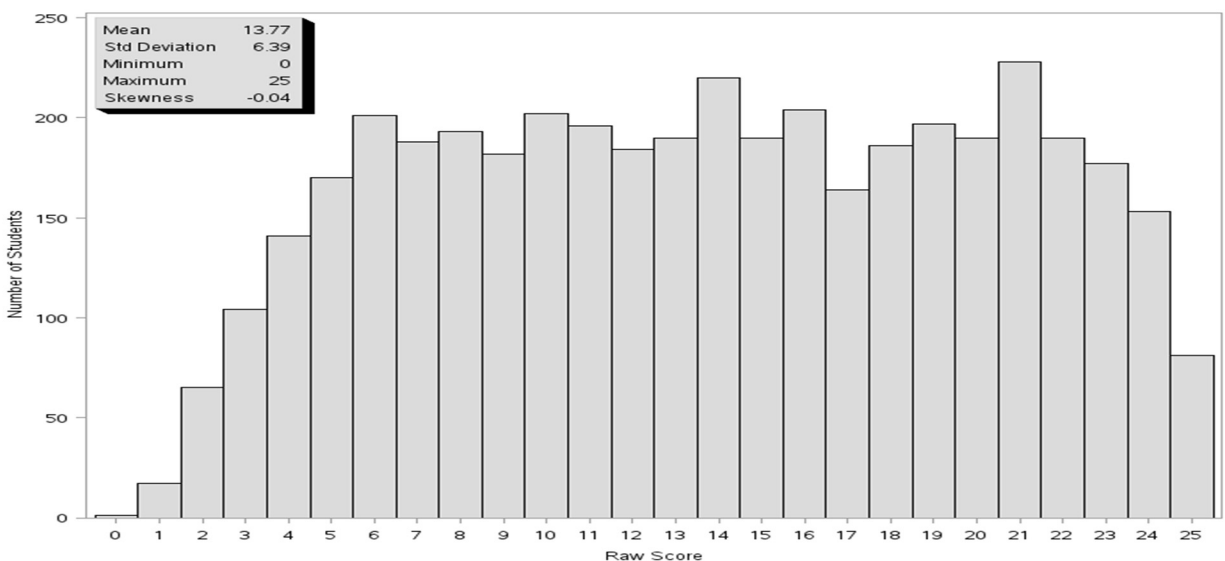
Figure 10. Raw score frequency distribution—grade 5 math interim 2
